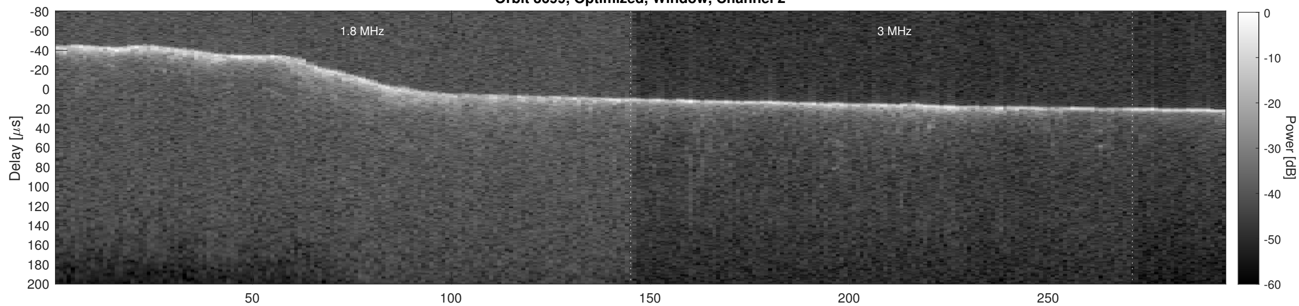
Orbit 3699, Cluttergram
