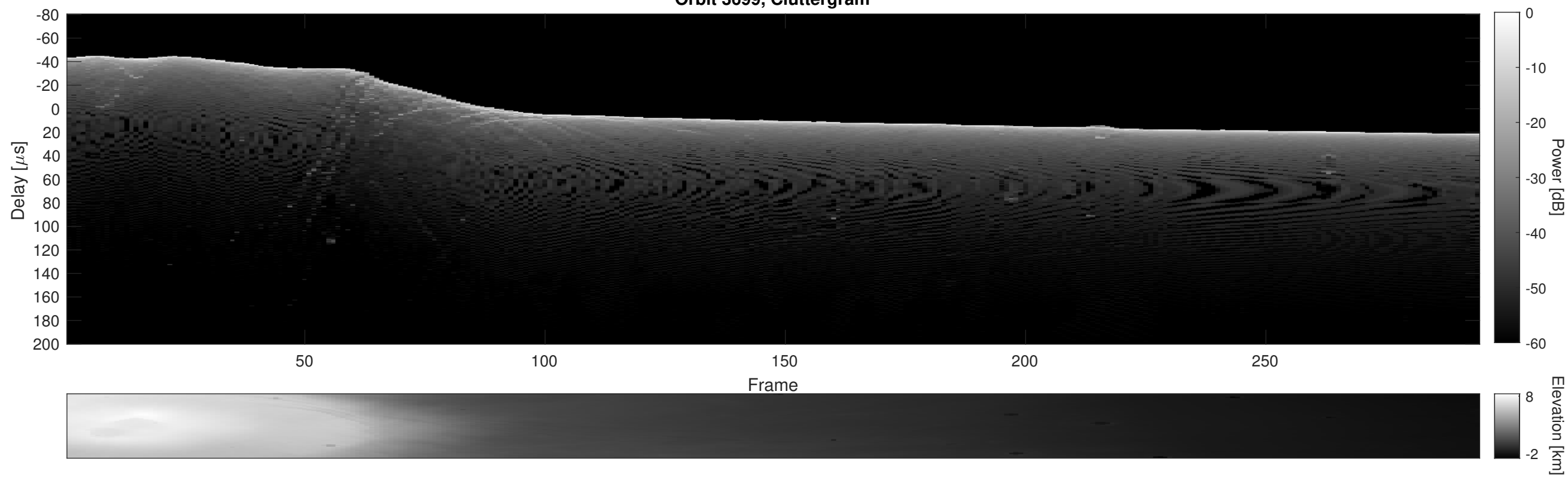
Orbit 3699, Cluttergram
