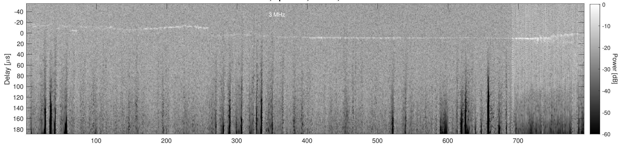
Orbit 3701, Cluttergram
