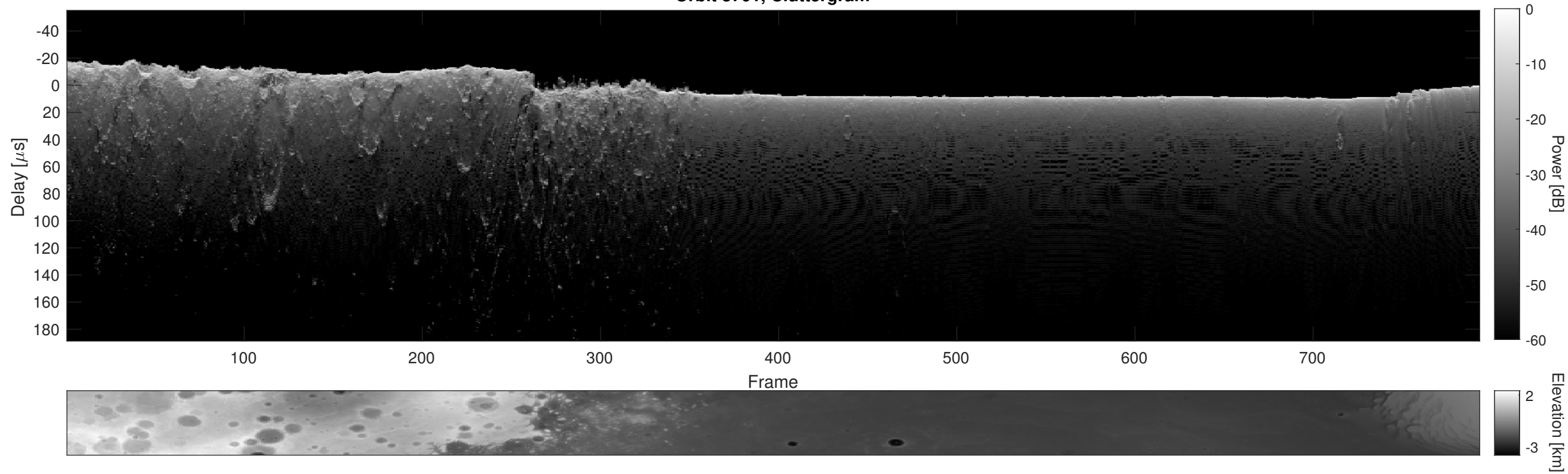
Orbit 3701, Cluttergram
