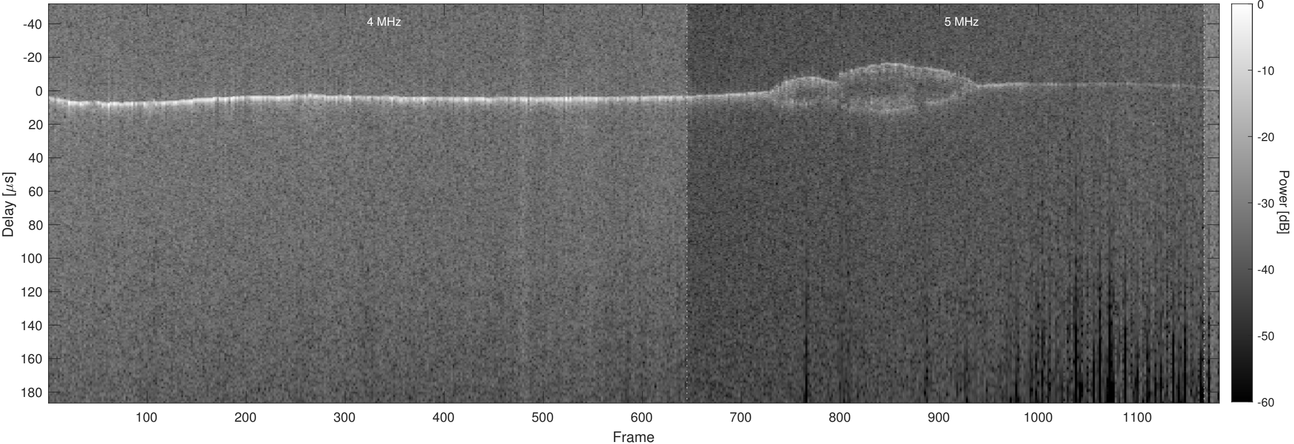
Orbit 3702, Optimized, No Window, Channel 2
