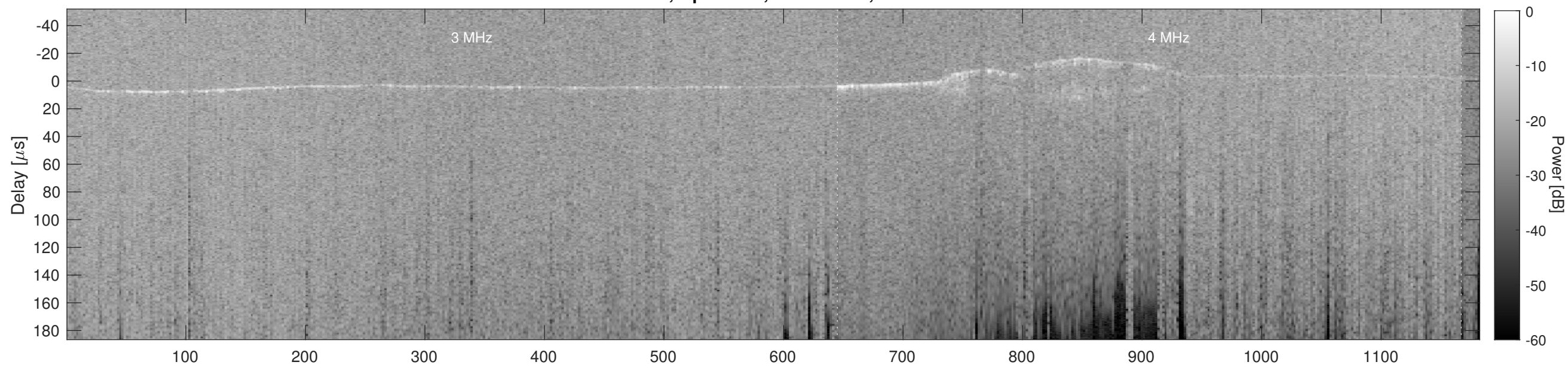
Orbit 3702, Cluttergram
