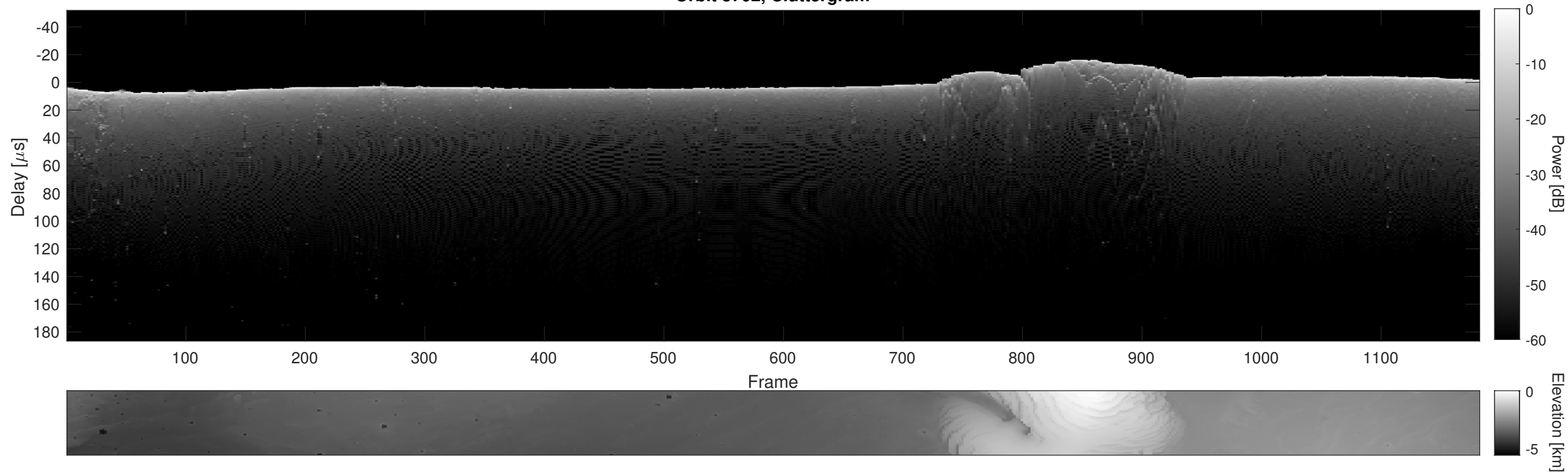
Orbit 3702, Cluttergram
