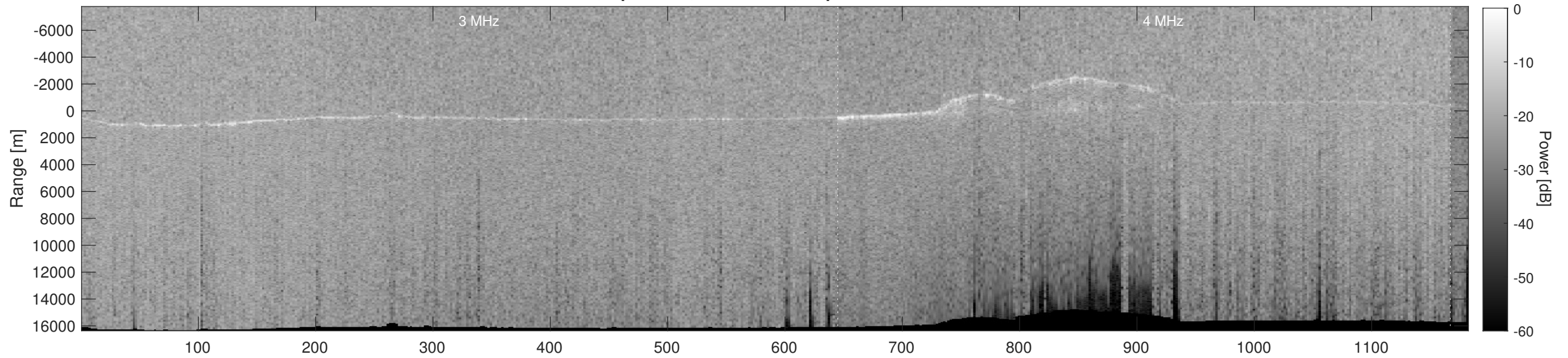
Orbit 3702, Depth-Corrected Cluttergram
