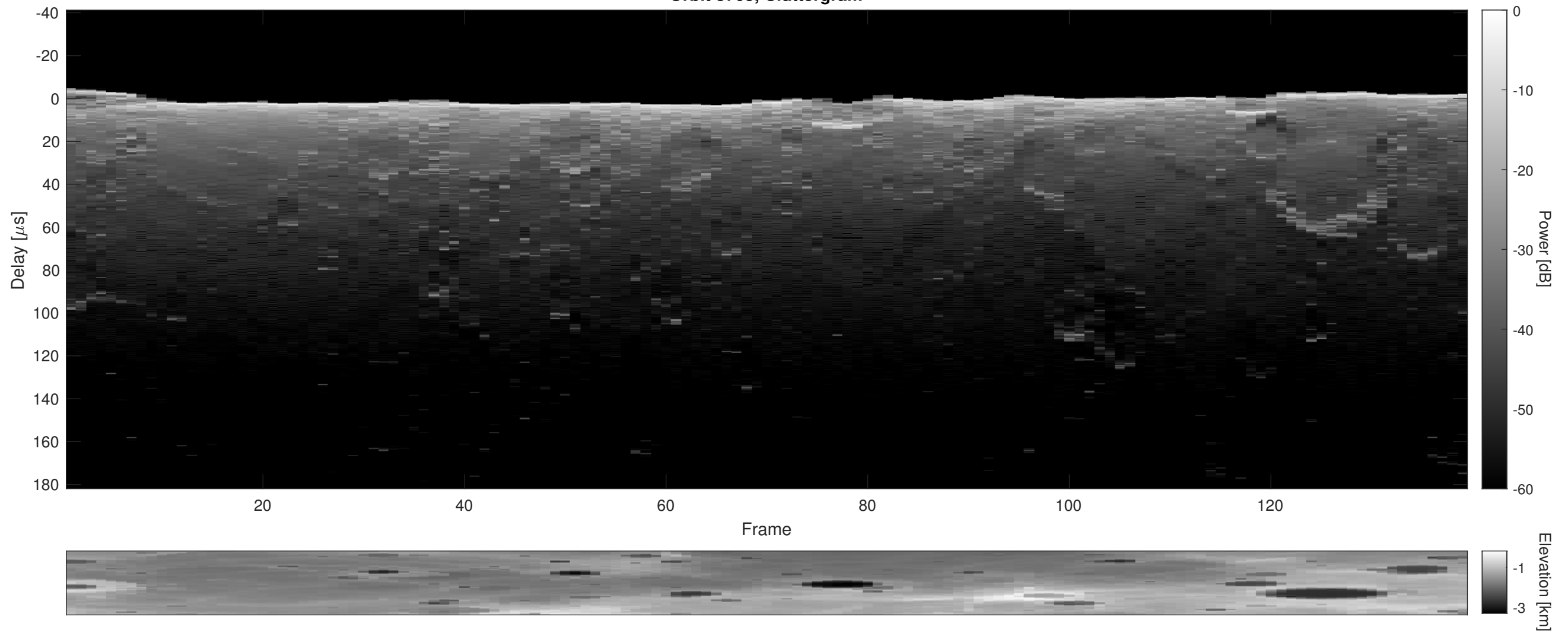
Orbit 3705, Cluttergram
