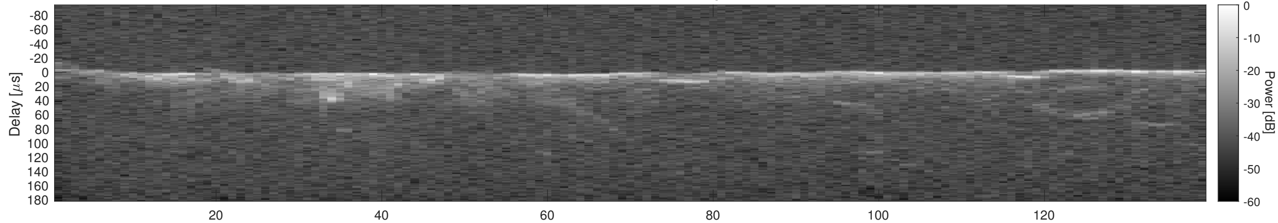
Orbit 3705, Cluttergram
