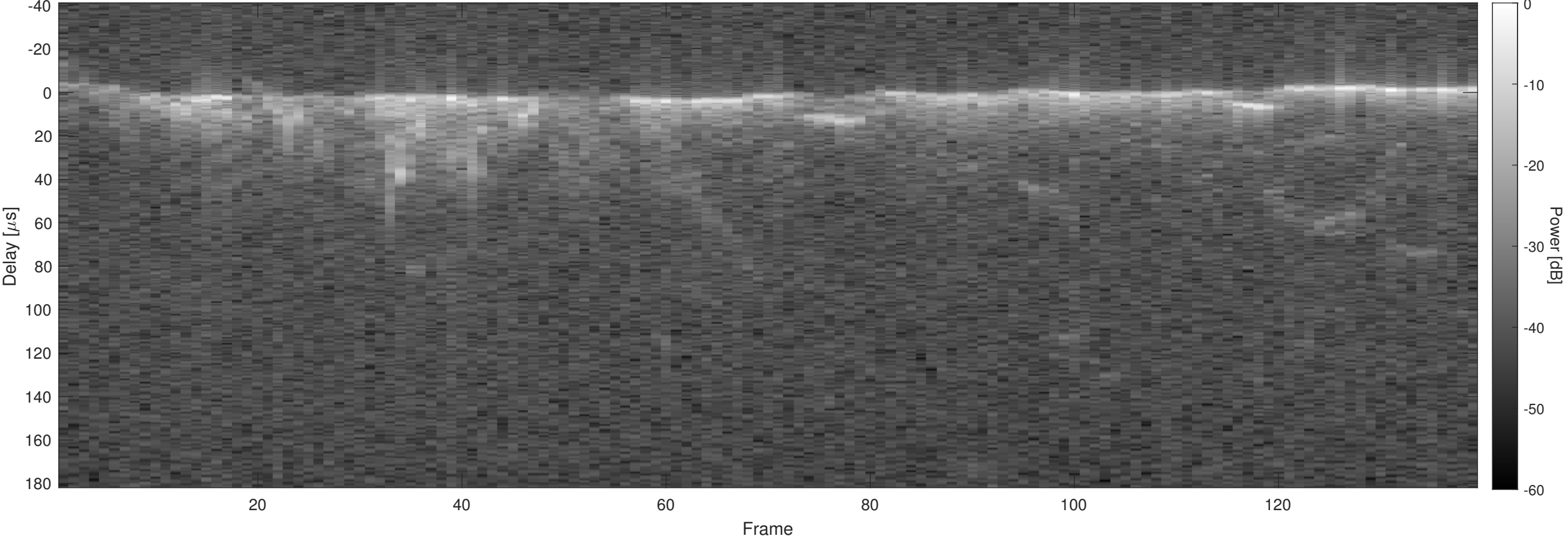
Orbit 3705, Optimized, No Window, Channel 2
