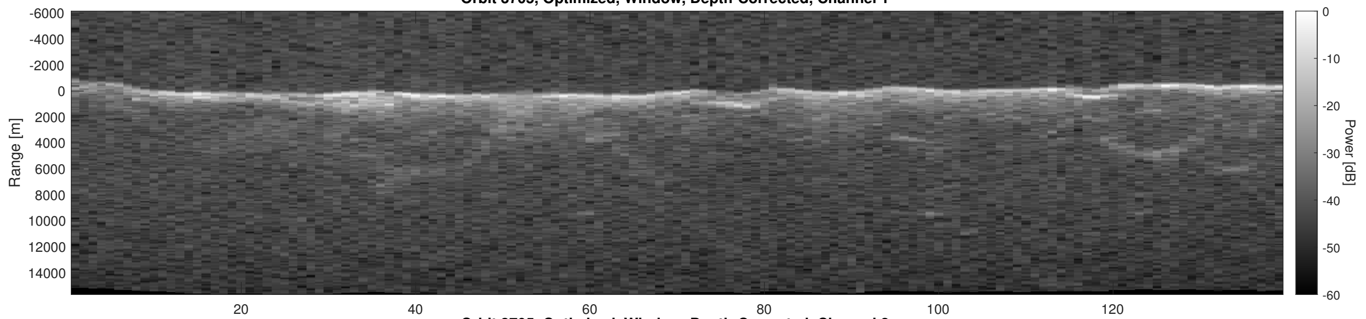
Orbit 3705, Optimized, Window, Depth-Corrected, Channel 2
