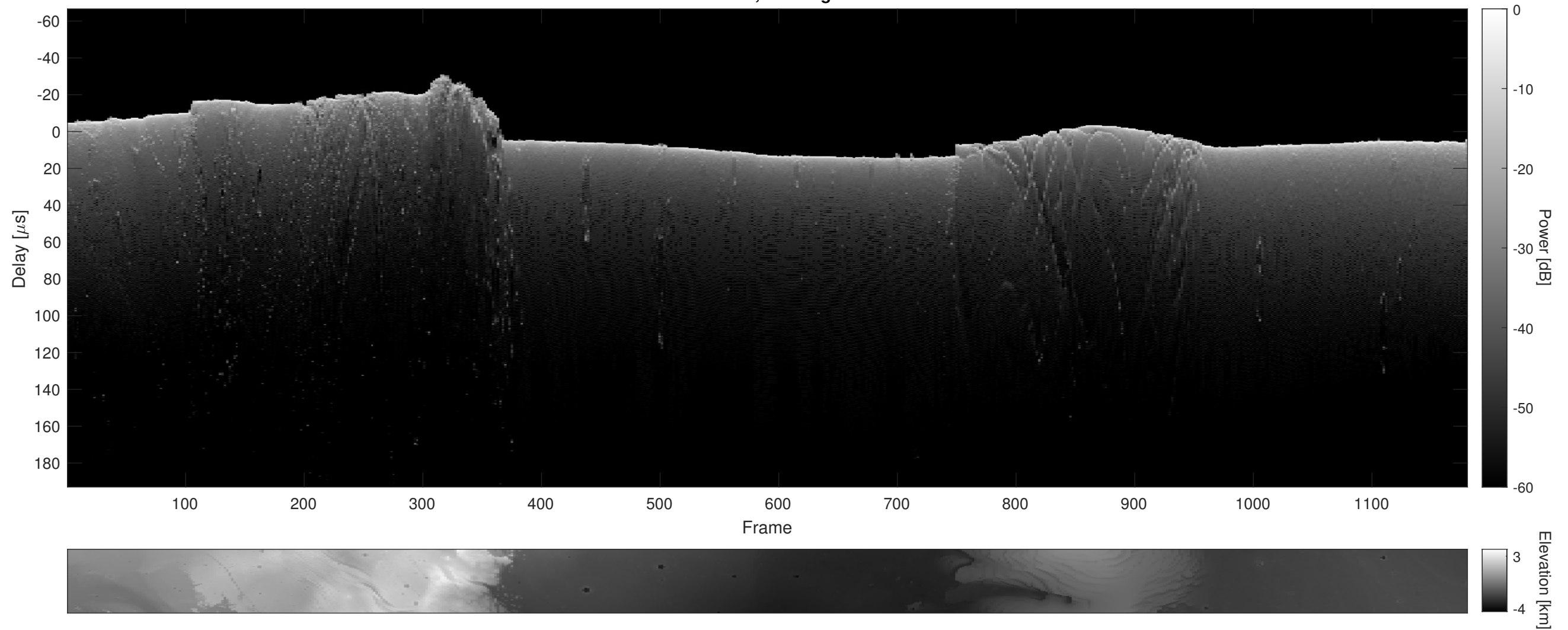
Orbit 3706, Cluttergram
