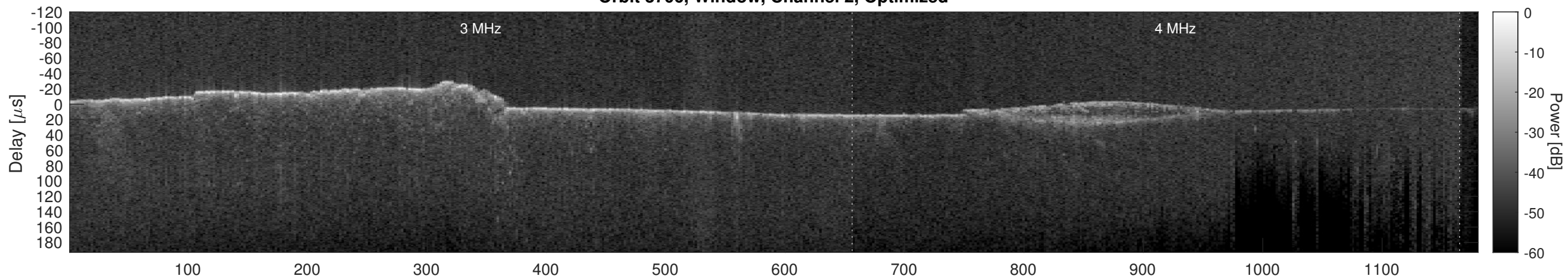
Orbit 3706, Cluttergram
