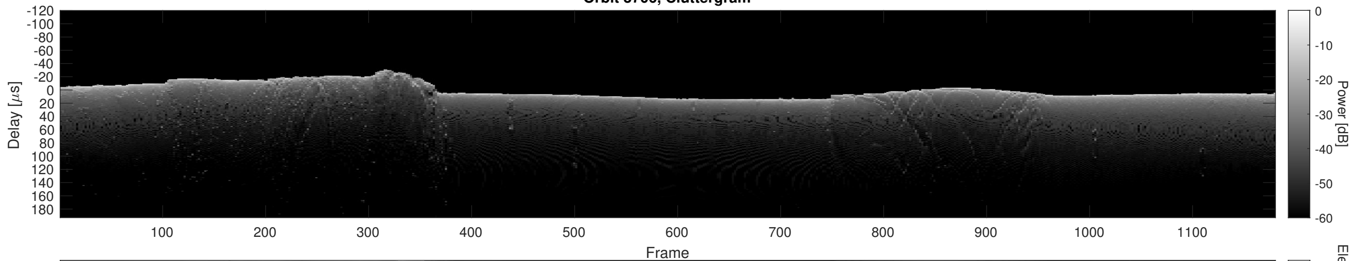
Orbit 3706, Cluttergram
