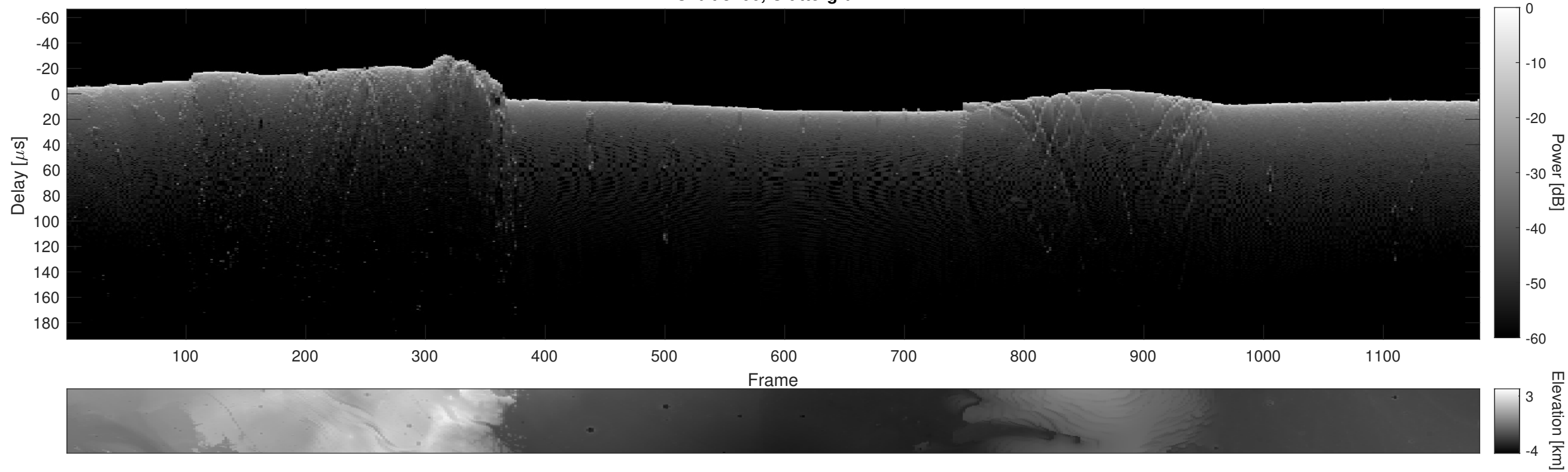
Orbit 3706, Cluttergram
