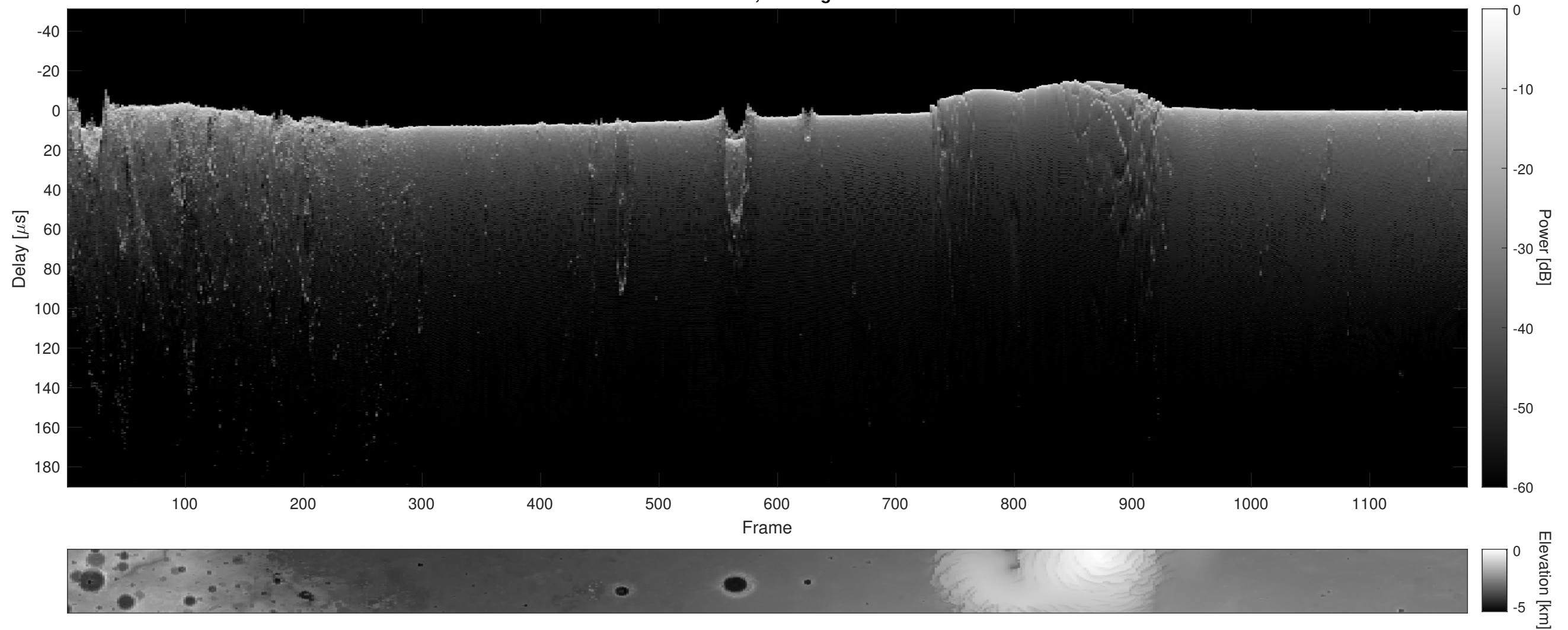
Orbit 3709, Cluttergram
