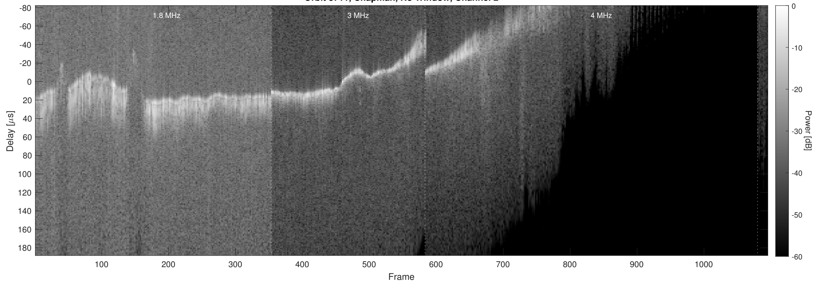
Orbit 3711, Chapman, No Window, Channel 2
