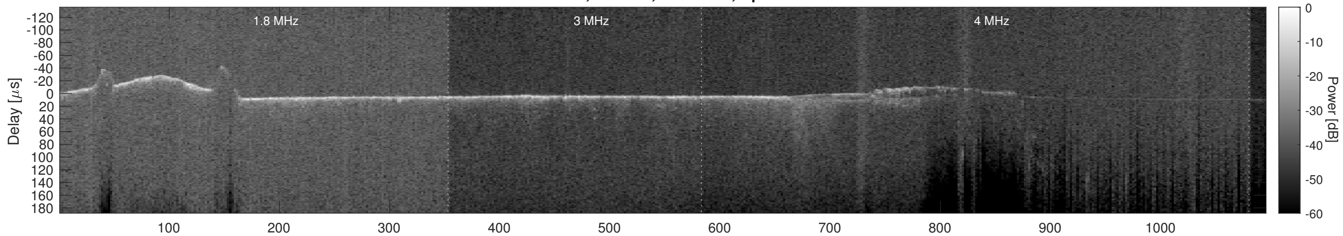
Orbit 3711, Cluttergram
