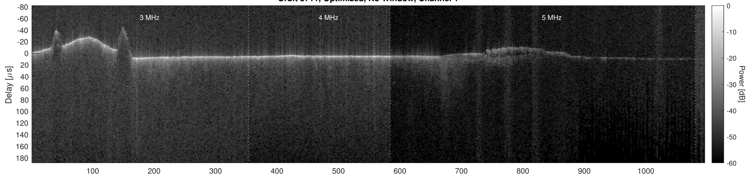
Orbit 3711, Optimized, No Window, Channel 2
