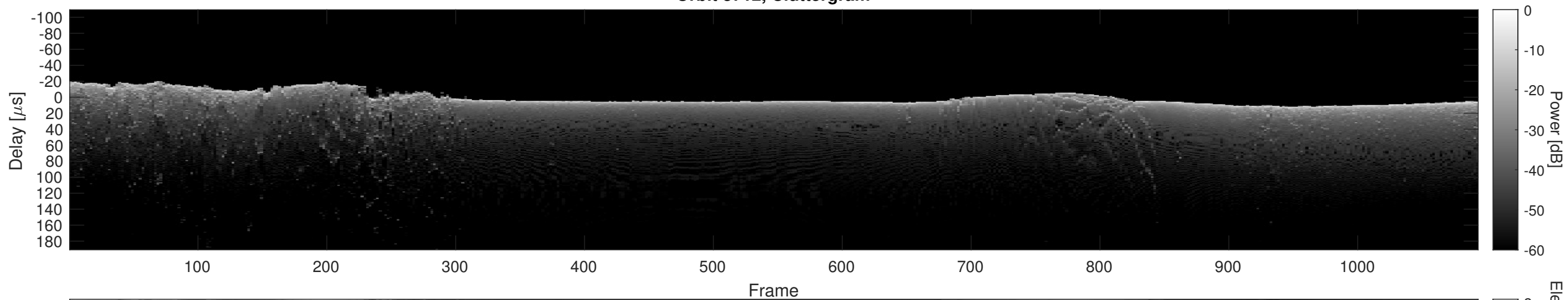
Orbit 3712, Cluttergram
