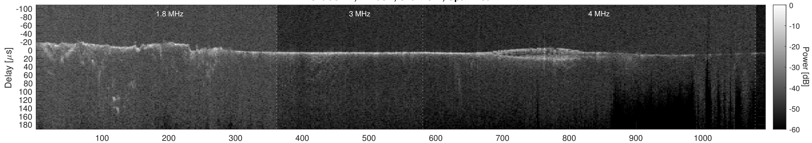
Orbit 3712, Cluttergram
