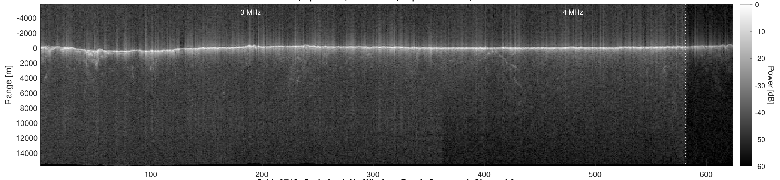
Orbit 3713, Optimized, No Window, Depth-Corrected, Channel 2
