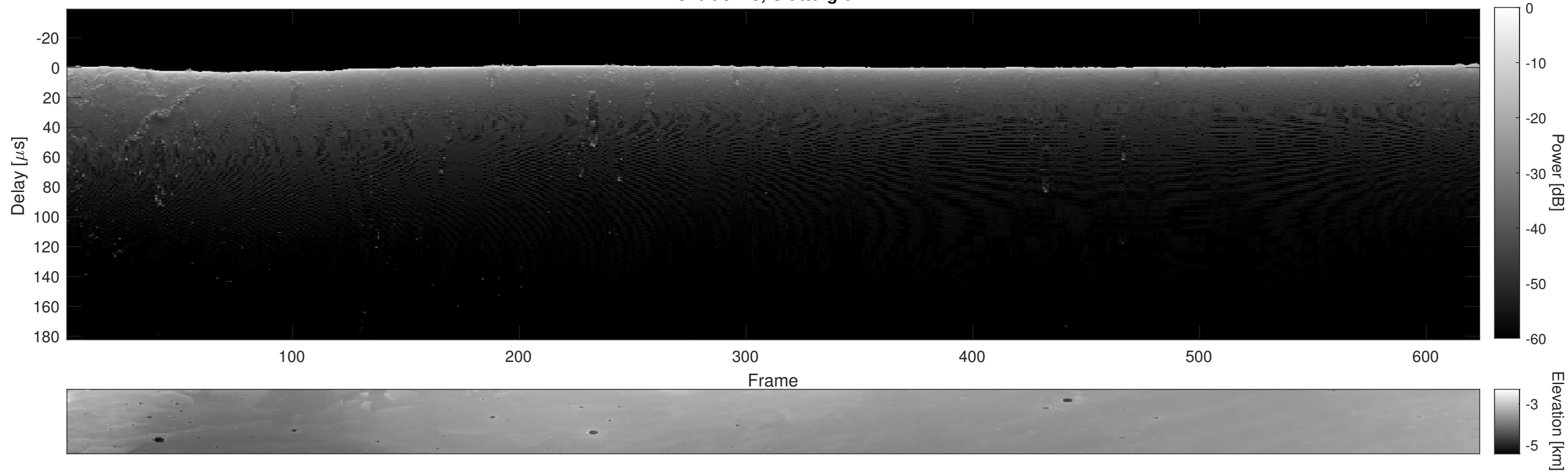
Orbit 3713, Cluttergram
