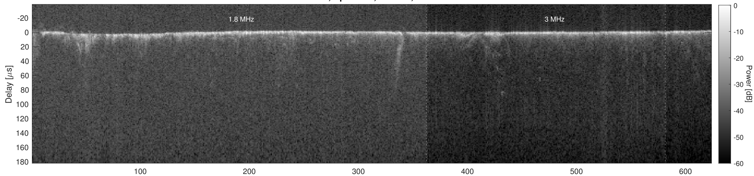
Orbit 3713, Cluttergram
