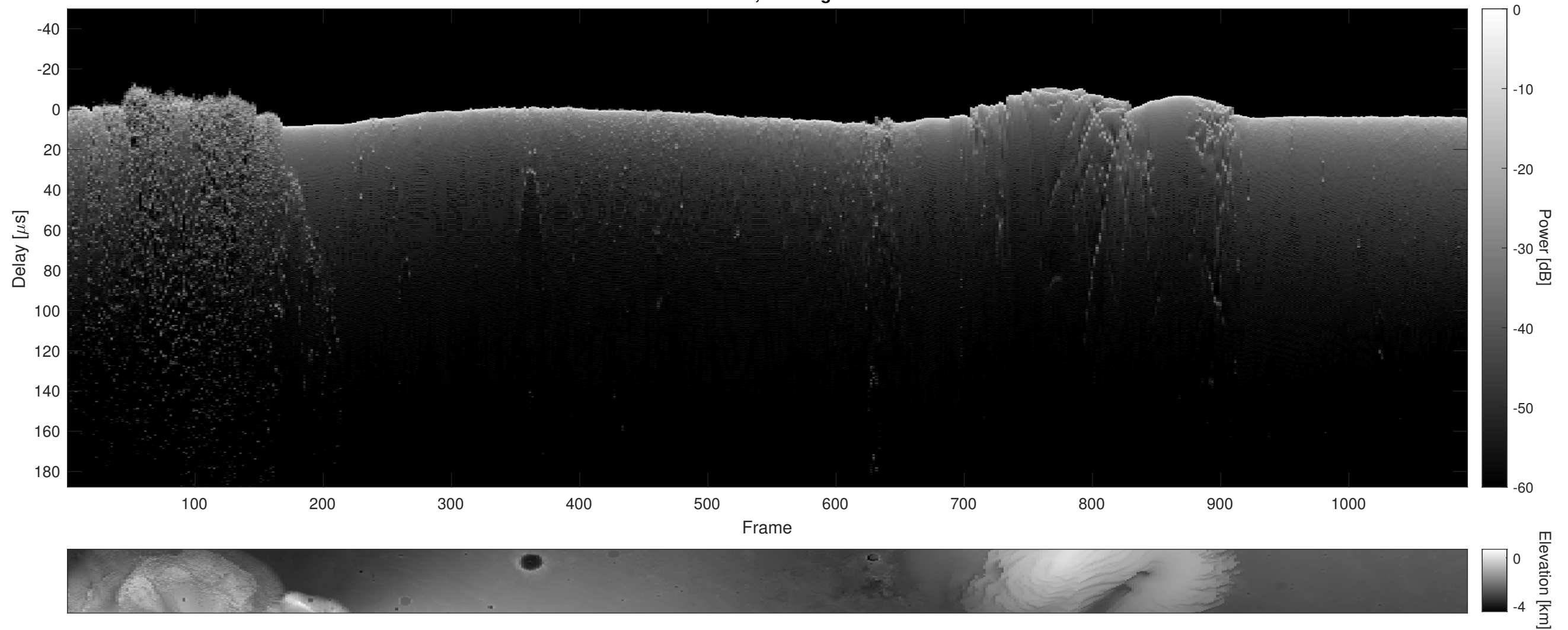
Orbit 3714, Cluttergram
