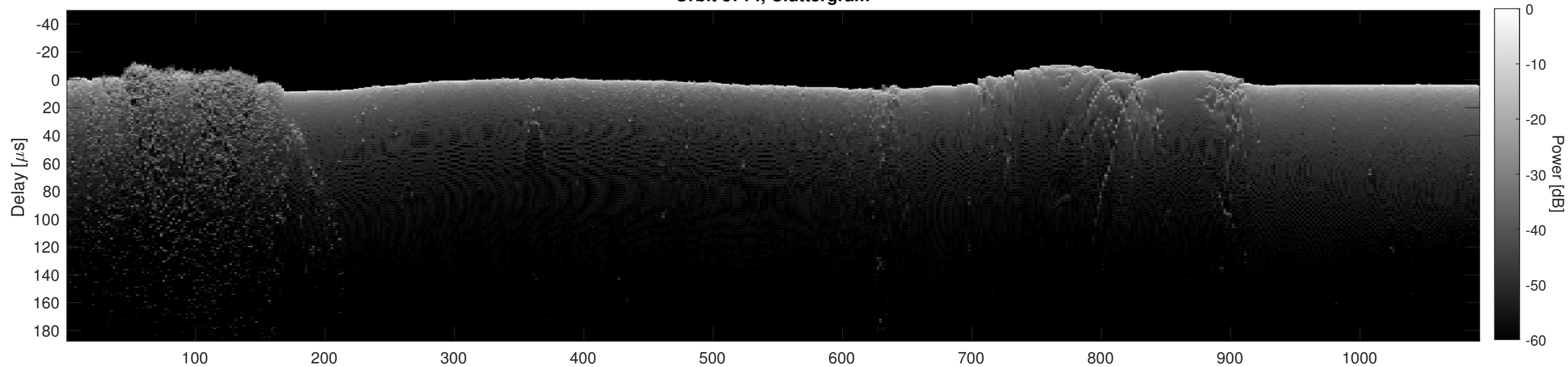
Orbit 3714, Cluttergram
