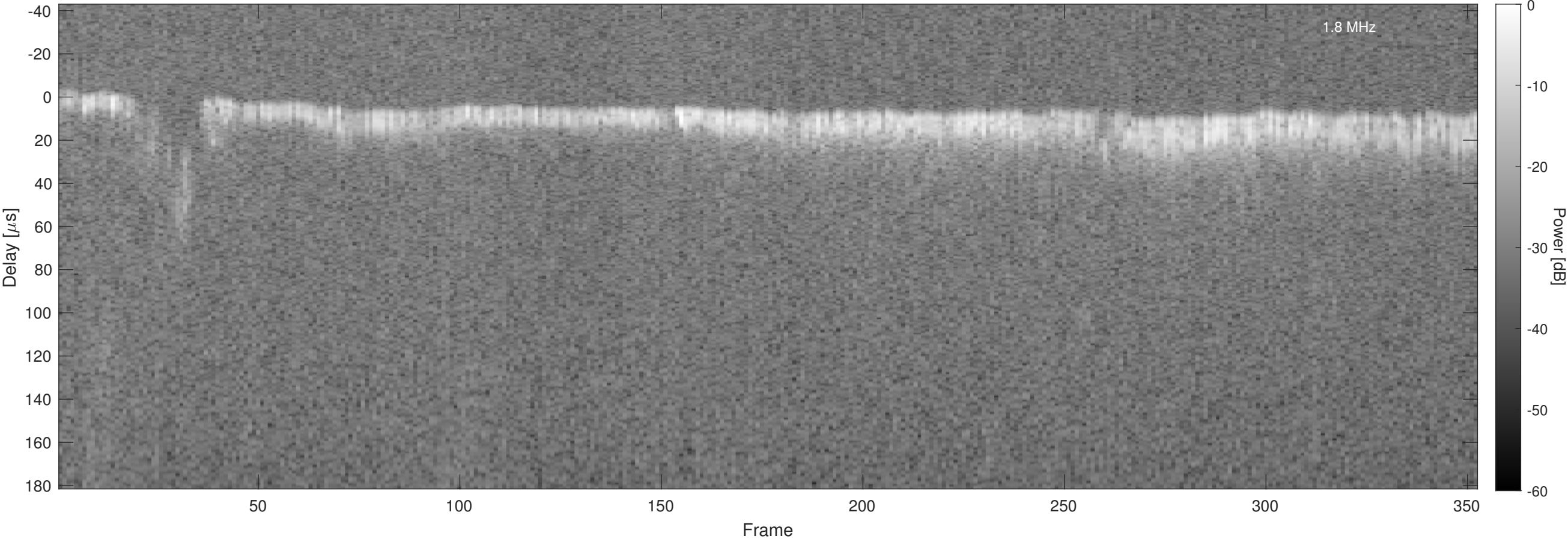
Orbit 3715, Chapman, Window, Channel 2
