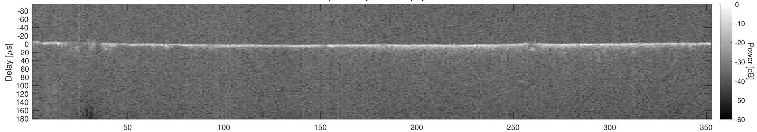
Orbit 3715, Cluttergram
