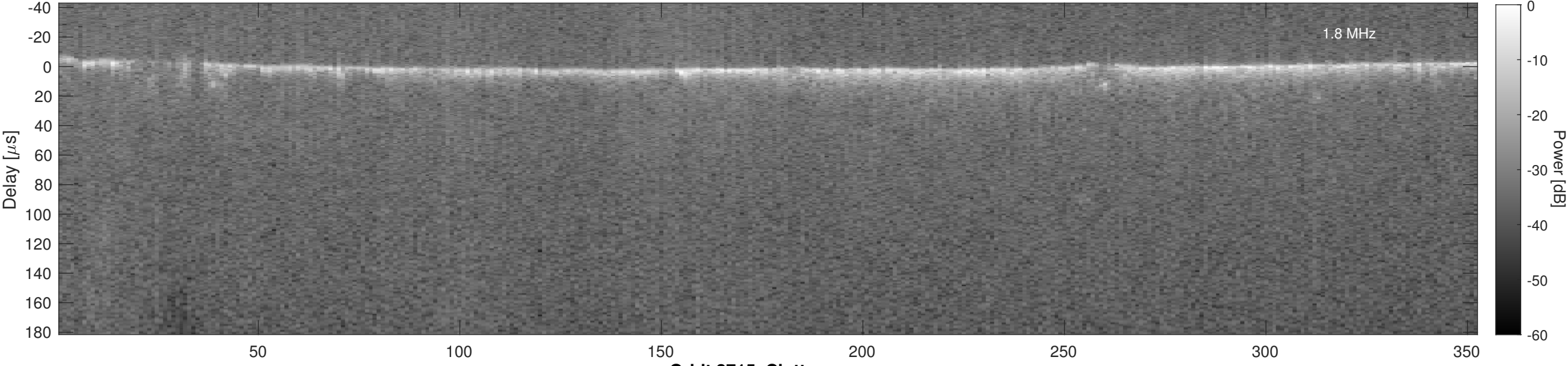
Orbit 3715, Cluttergram
