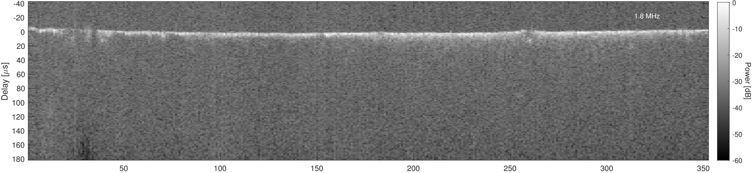
Orbit 3715, Cluttergram
