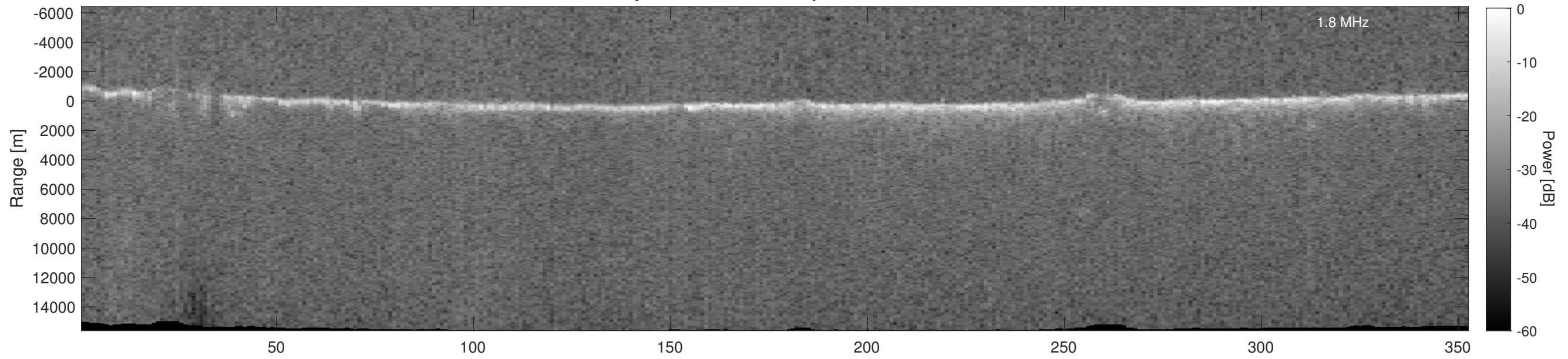
Orbit 3715, Depth-Corrected Cluttergram
