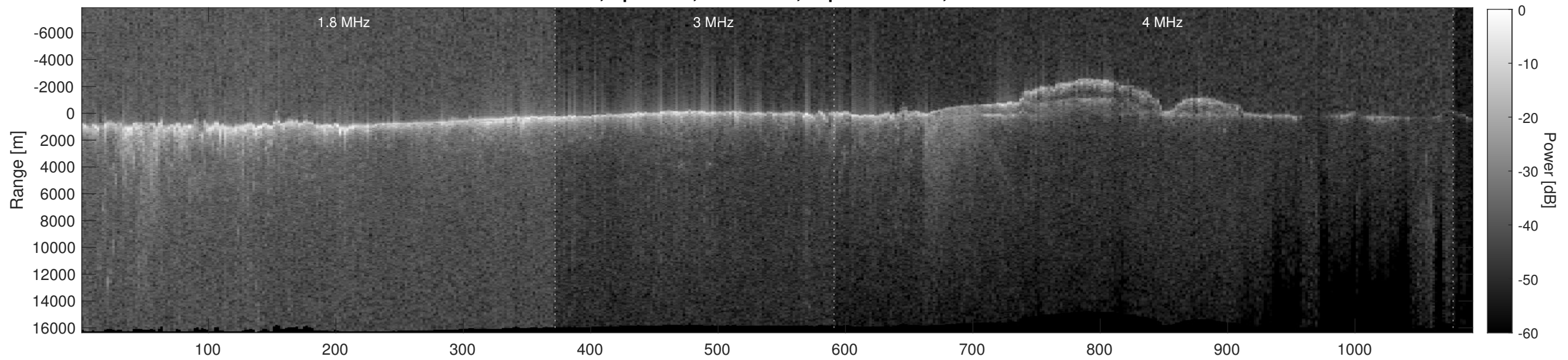
Orbit 3718, Depth-Corrected Cluttergram
