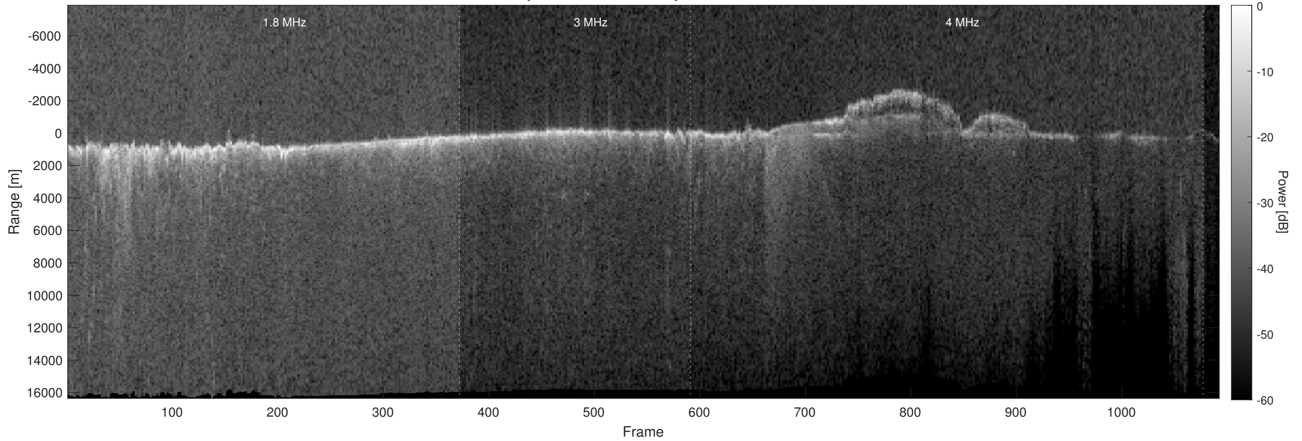
Orbit 3718, Optimized, Window, Depth-Corrected, Channel 2
