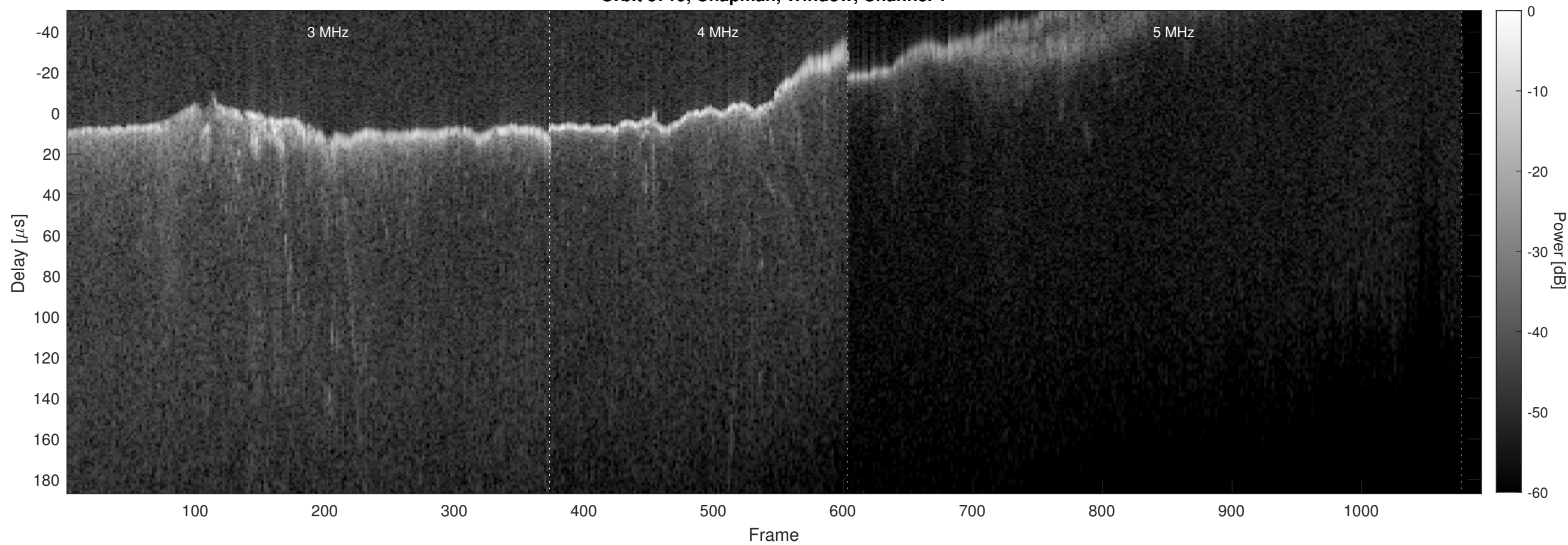
Orbit 3719, Chapman, Window, Channel 2
