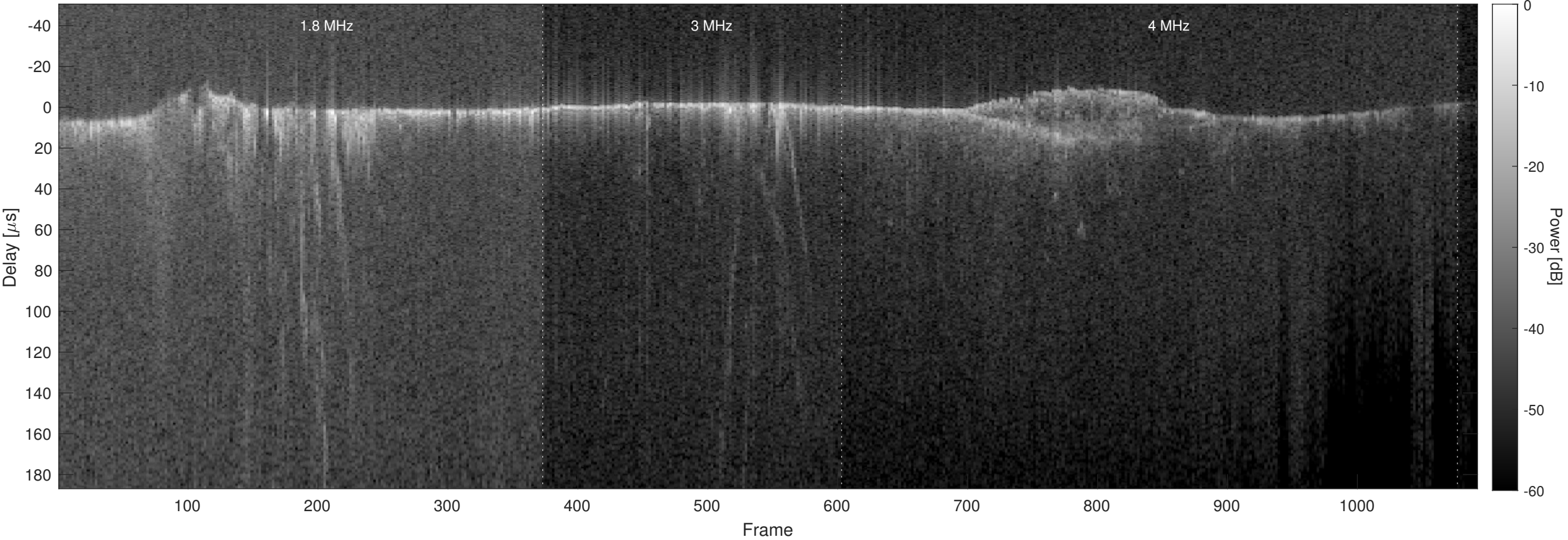
Orbit 3719, Optimized, No Window, Channel 2
