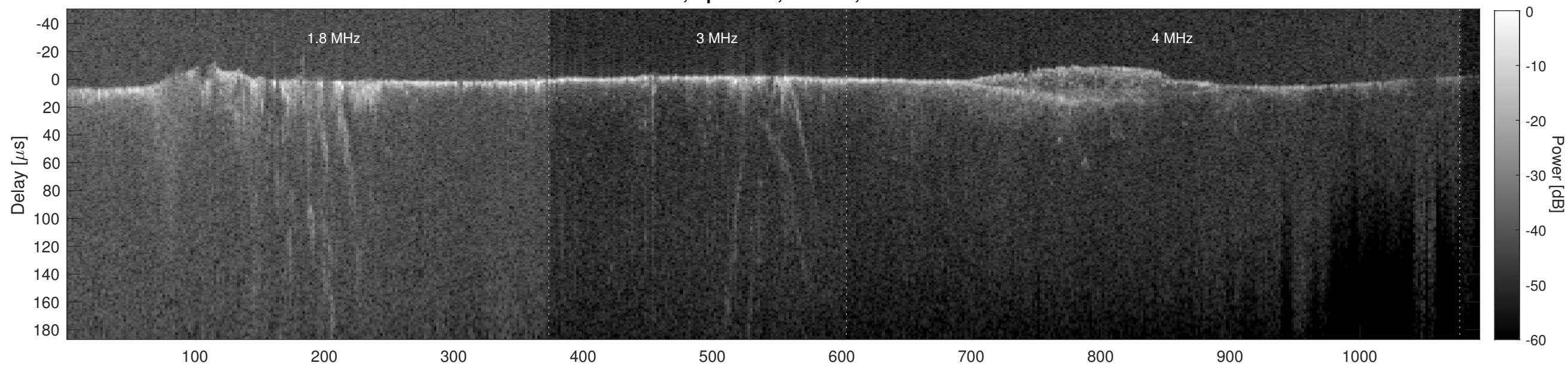
Orbit 3719, Cluttergram
