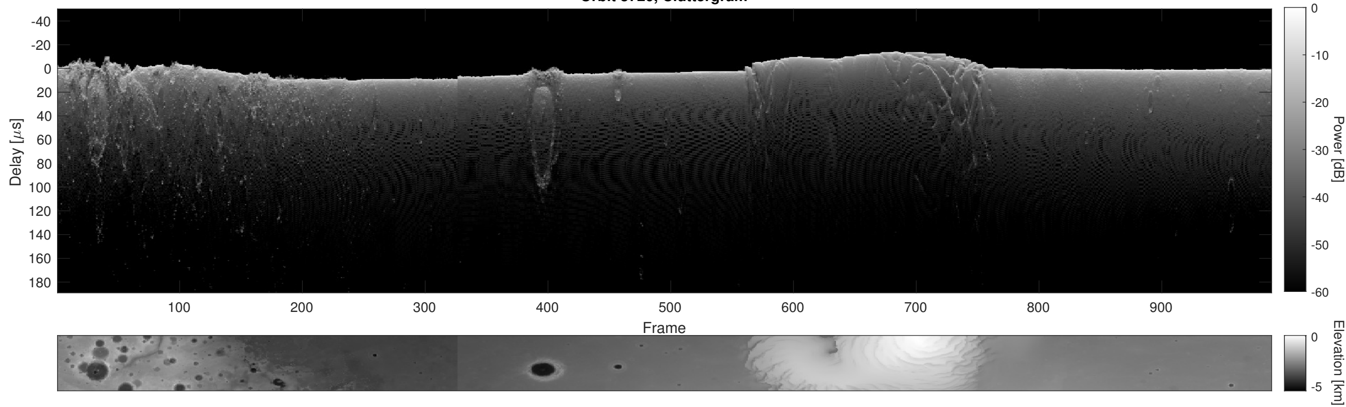
Orbit 3720, Cluttergram
