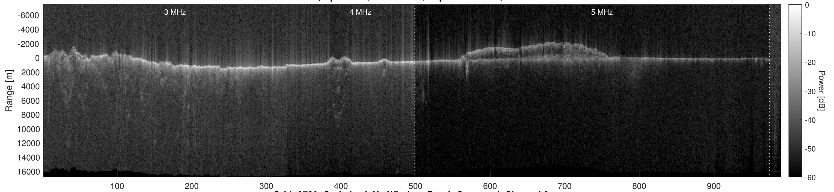
Orbit 3720, Optimized, No Window, Depth-Corrected, Channel 2
