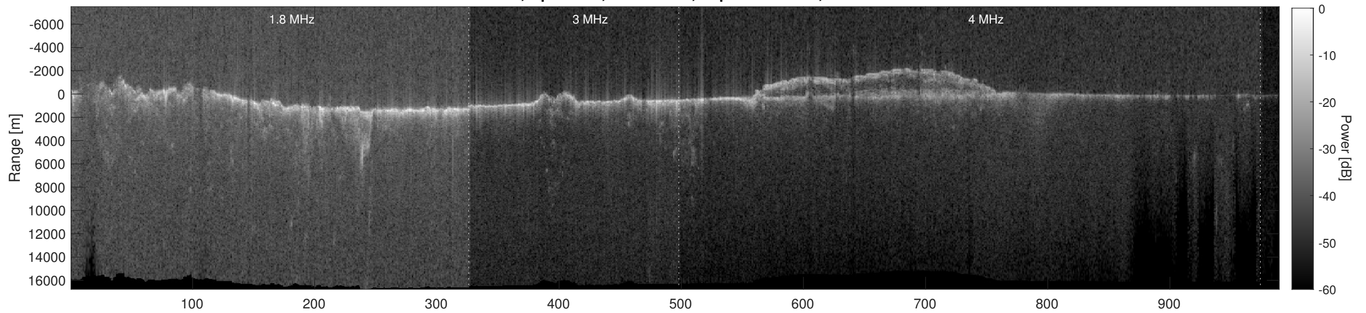
Orbit 3720, Depth-Corrected Cluttergram
