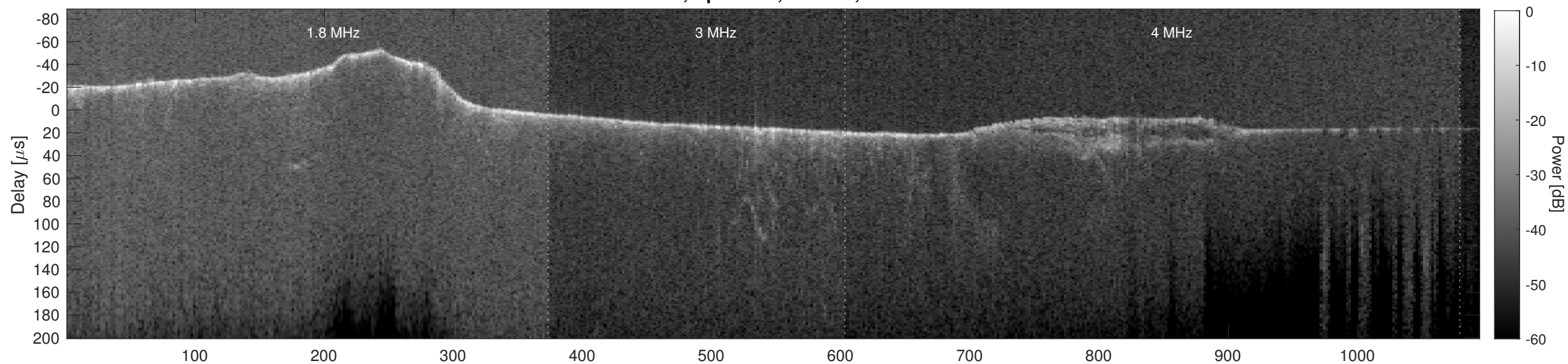
Orbit 3721, Cluttergram
