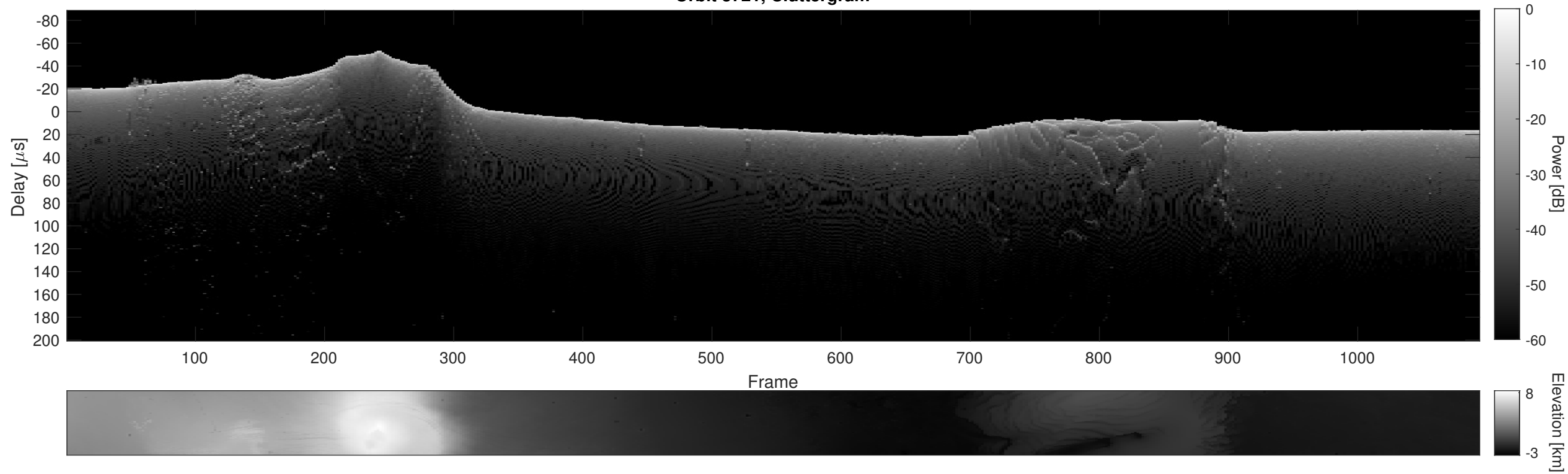
Orbit 3721, Cluttergram
