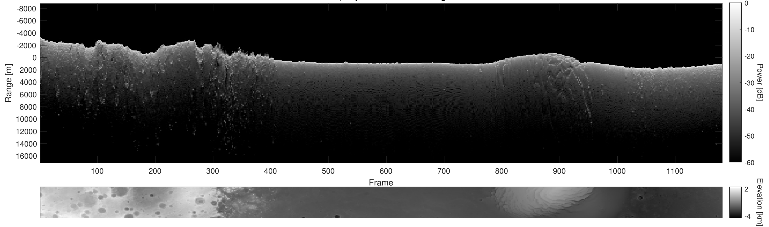
Orbit 3723, Depth-Corrected Cluttergram
