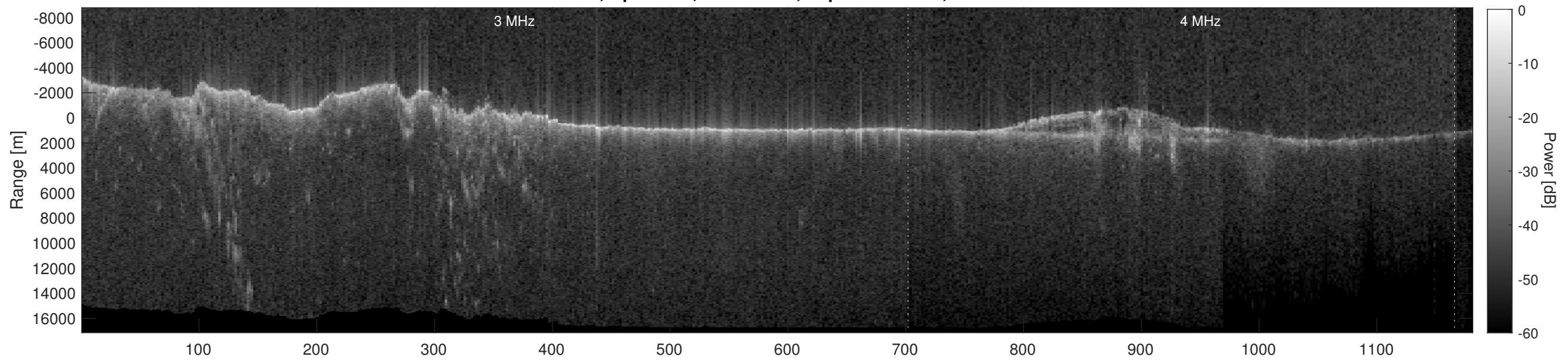
Orbit 3723, Depth-Corrected Cluttergram
