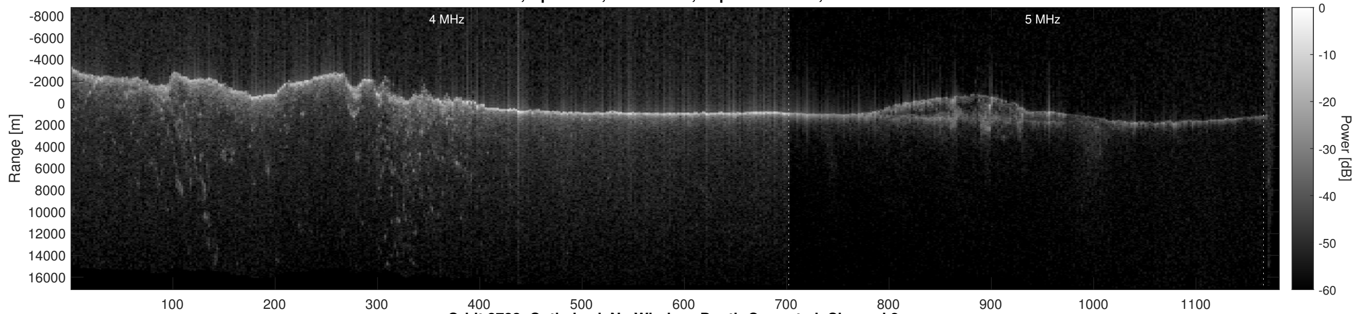
Orbit 3723, Optimized, No Window, Depth-Corrected, Channel 2
