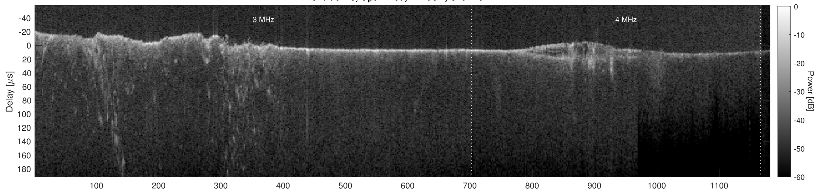
Orbit 3723, Cluttergram
