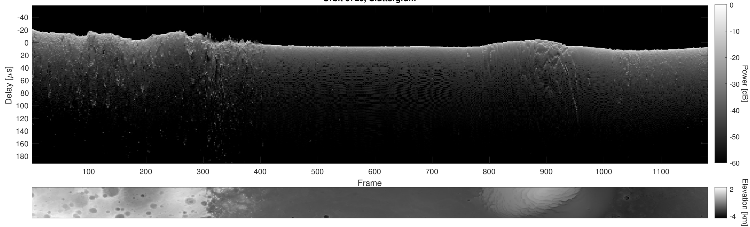
Orbit 3723, Cluttergram
