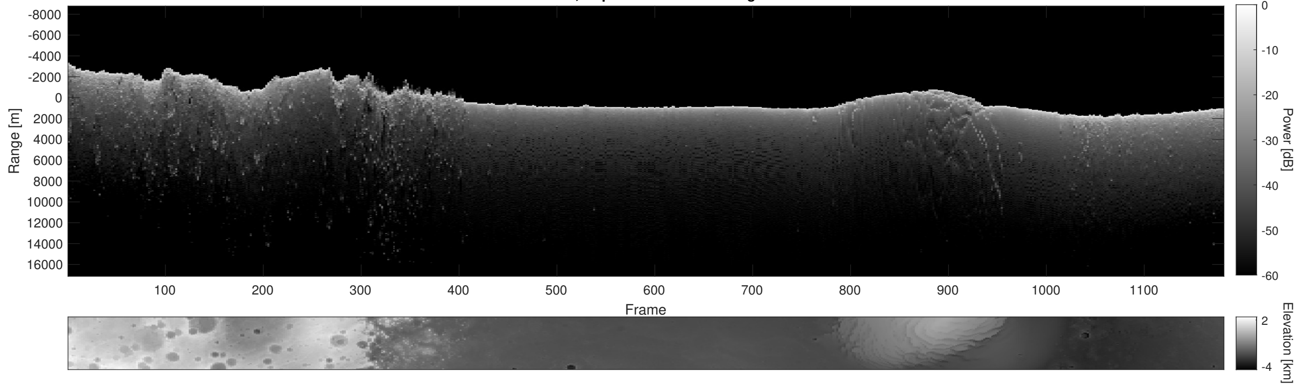
Orbit 3723, Depth-Corrected Cluttergram
