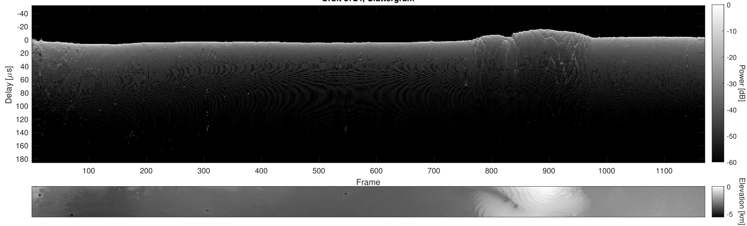
Orbit 3724, Cluttergram
