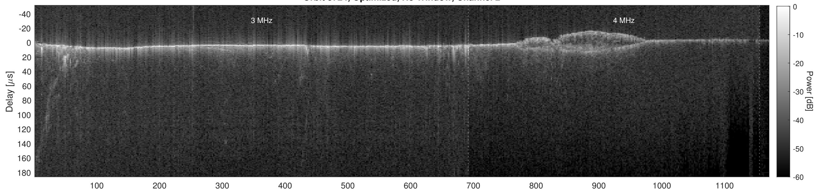
Orbit 3724, Cluttergram
