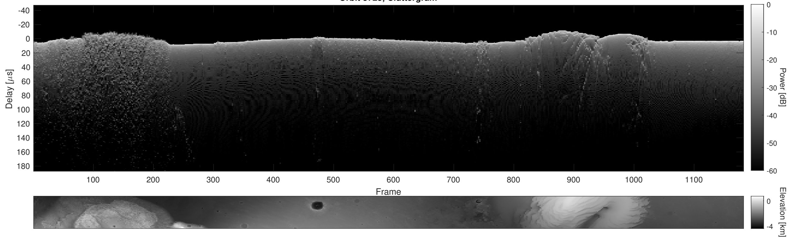
Orbit 3725, Cluttergram
