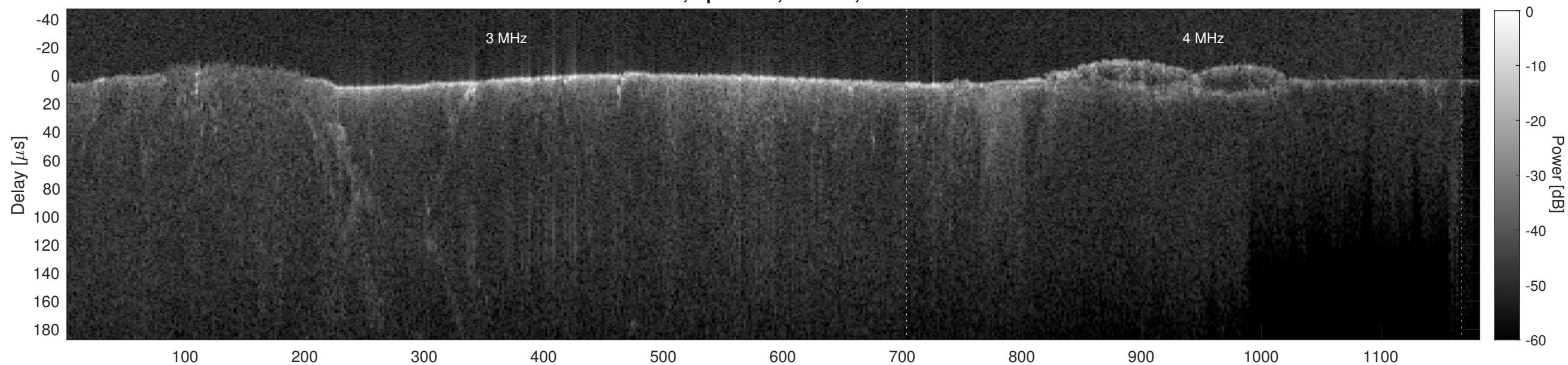
Orbit 3725, Cluttergram
