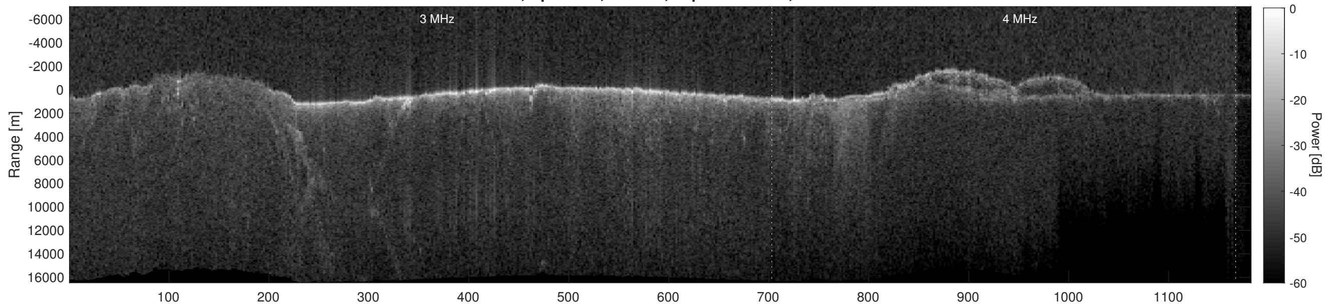
Orbit 3725, Depth-Corrected Cluttergram
