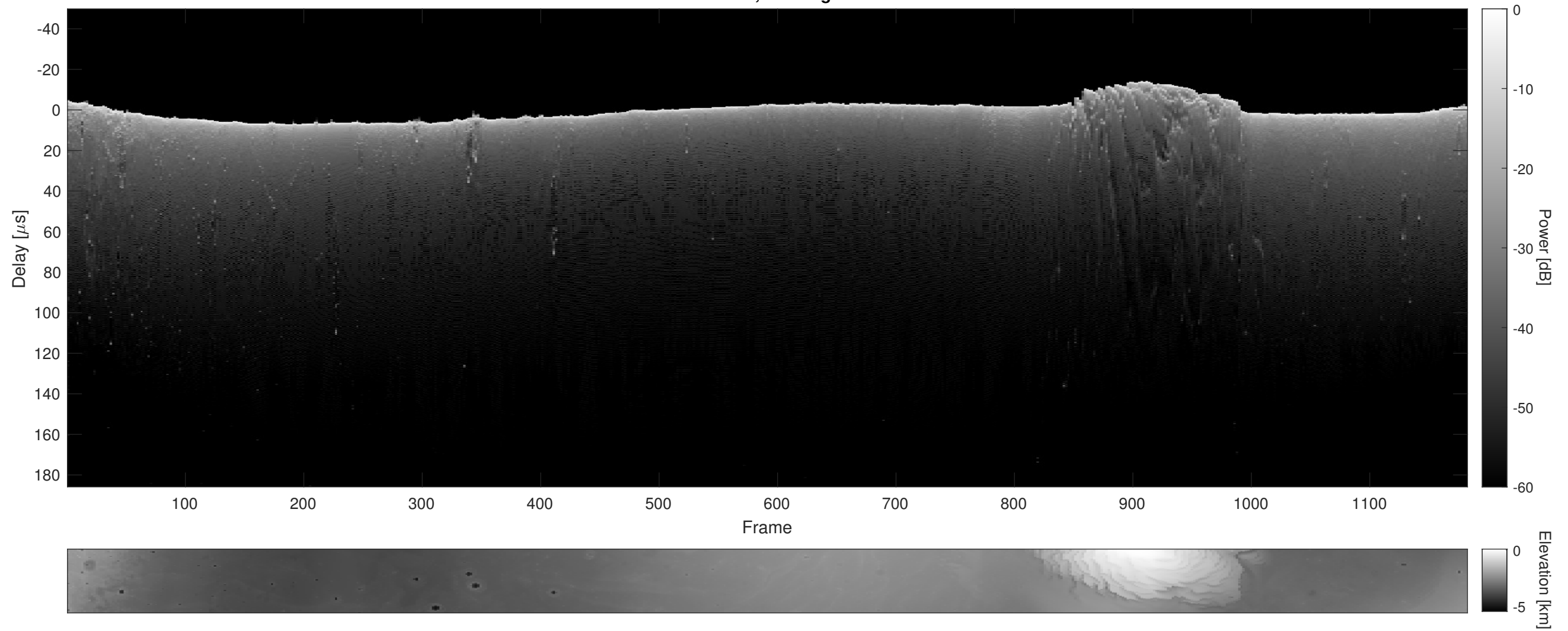
Orbit 3726, Cluttergram
