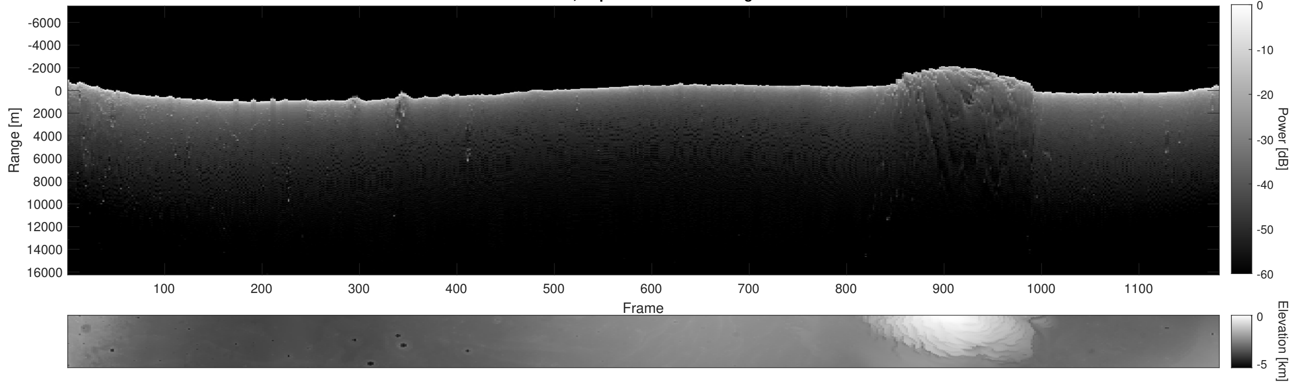
Orbit 3726, Depth-Corrected Cluttergram
