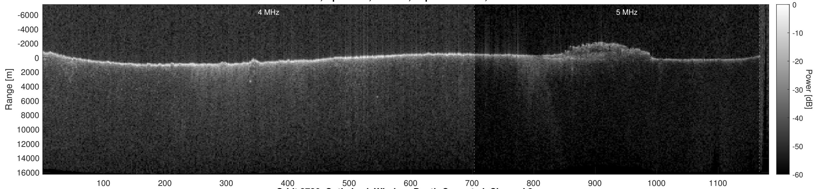
Orbit 3726, Optimized, Window, Depth-Corrected, Channel 2
