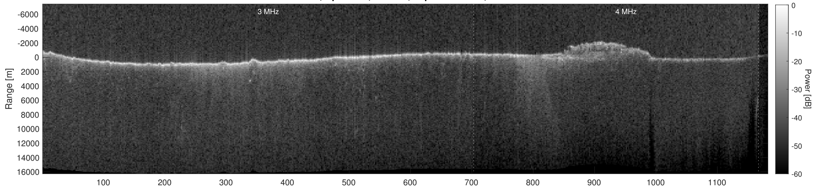
Orbit 3726, Depth-Corrected Cluttergram
