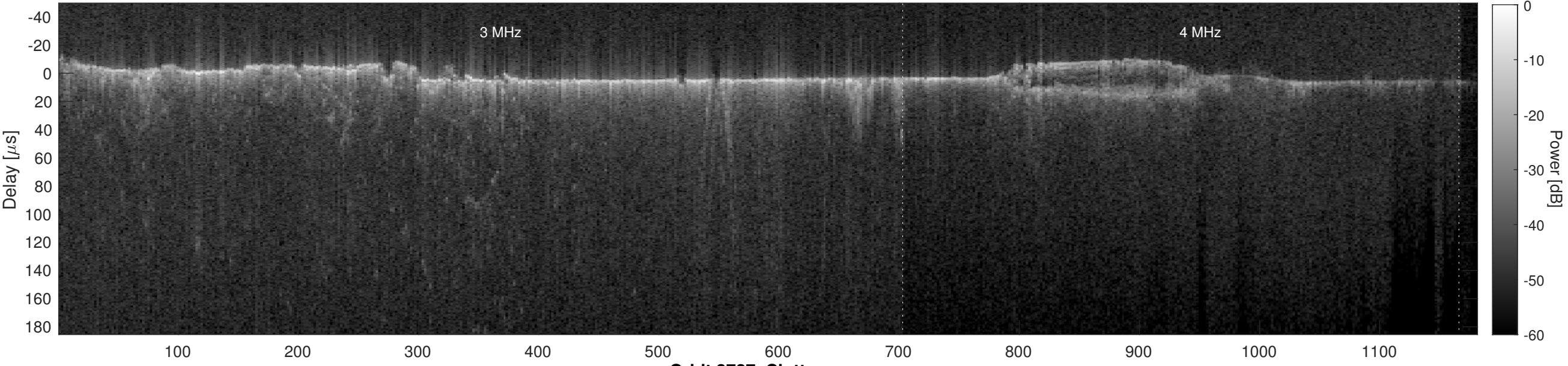
Orbit 3727, Cluttergram
