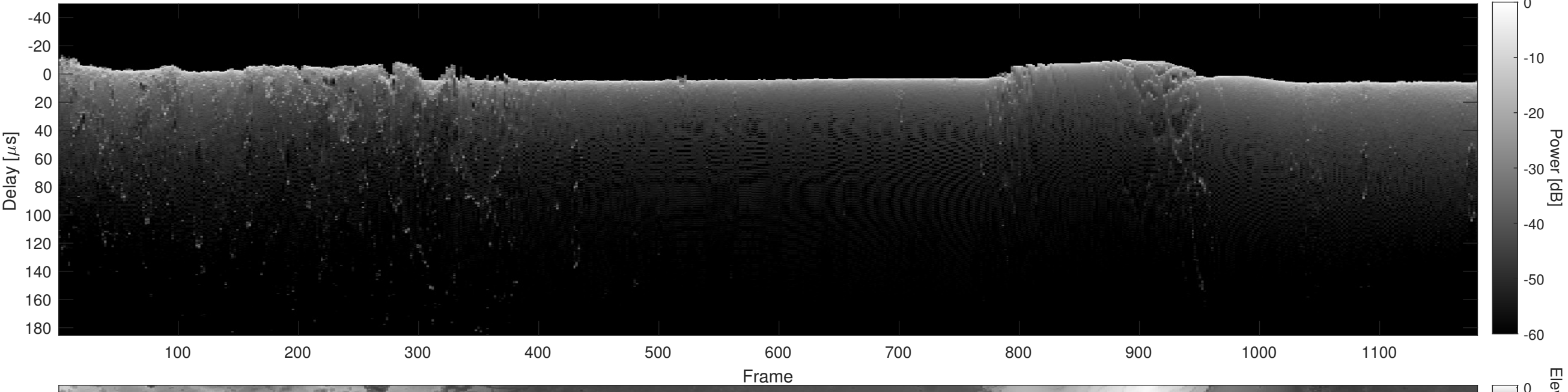
Orbit 3727, Cluttergram
