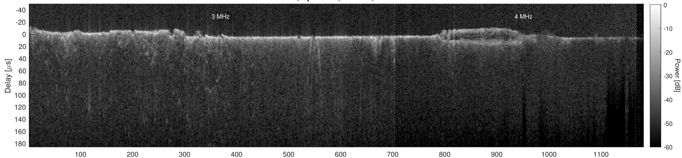
Orbit 3727, Cluttergram
