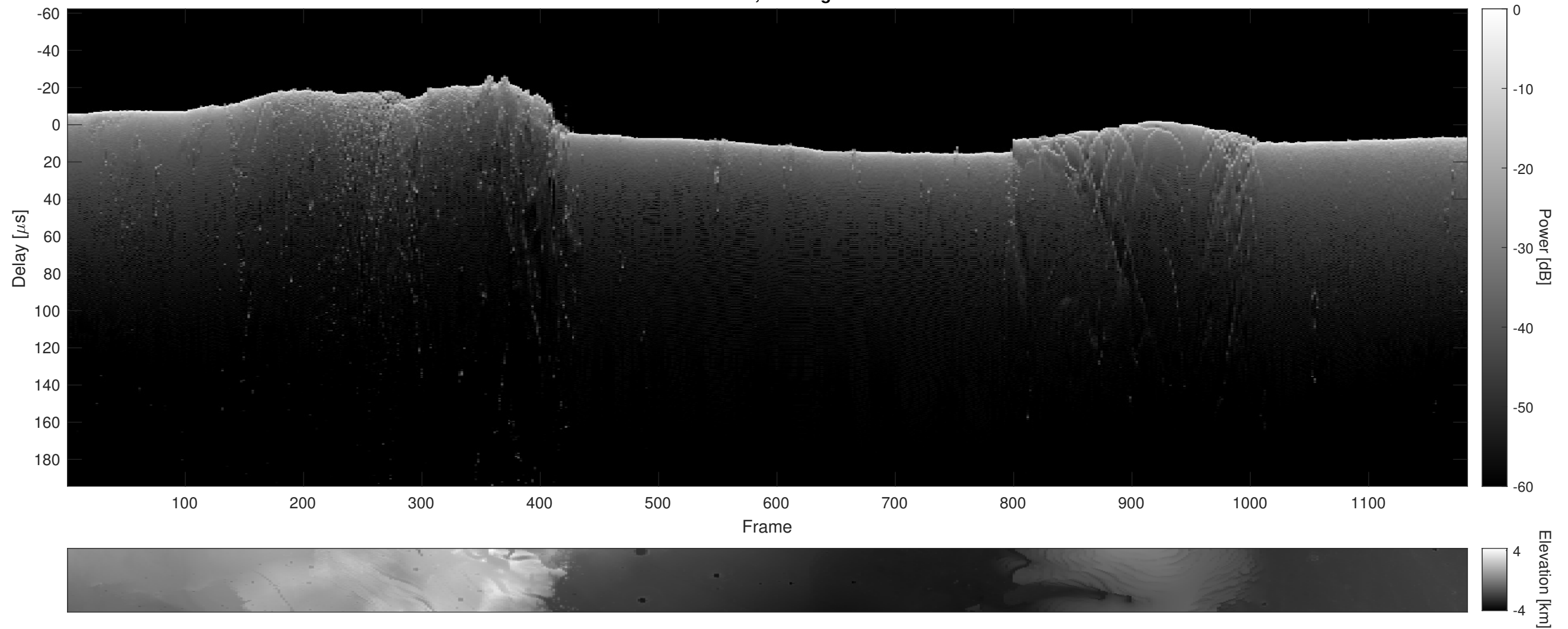
Orbit 3728, Cluttergram
