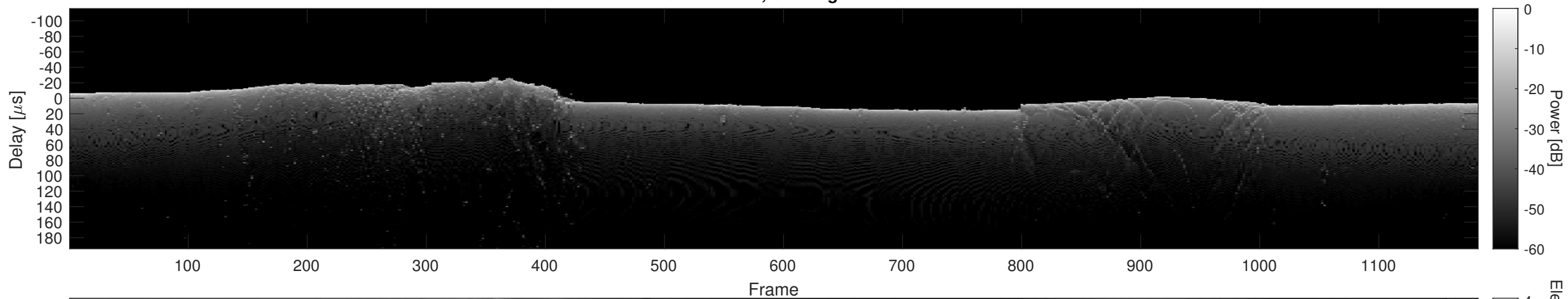
Orbit 3728, Cluttergram
