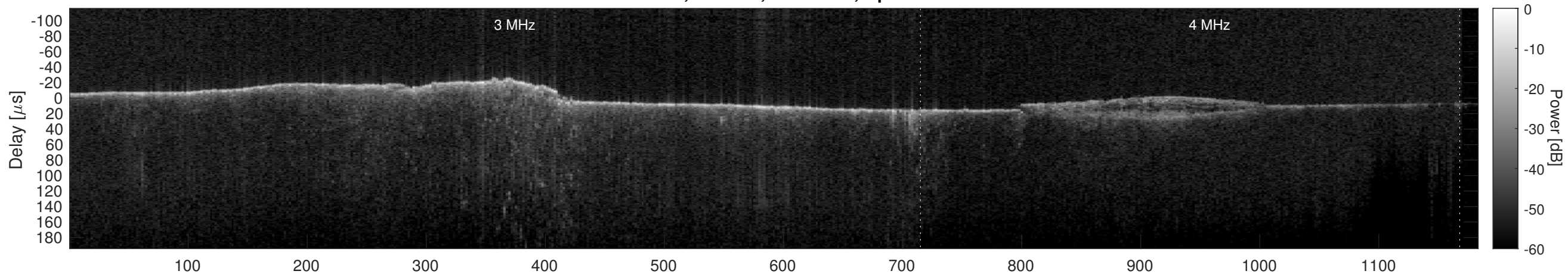
Orbit 3728, Cluttergram
