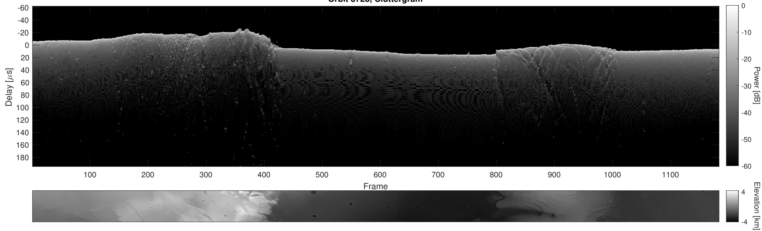
Orbit 3728, Cluttergram
