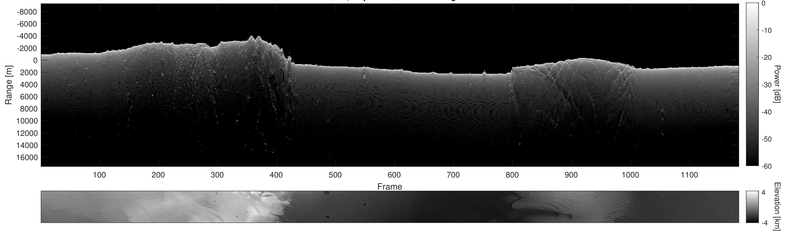
Orbit 3728, Depth-Corrected Cluttergram
