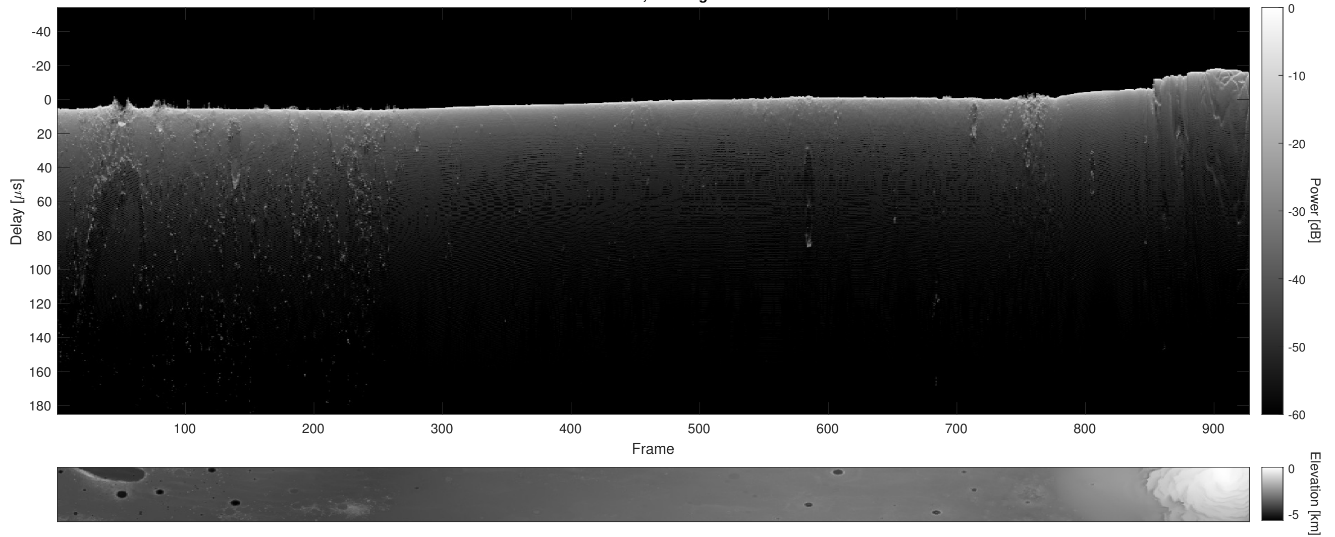
Orbit 3729, Cluttergram
